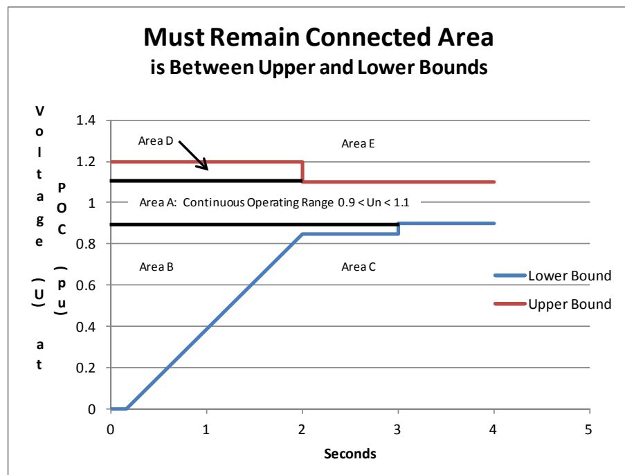
Figure 5-1: Voltage Must Remain Connected Area
